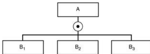
FIGURE 4.2.2(a) An Example of an “And” Gate.
