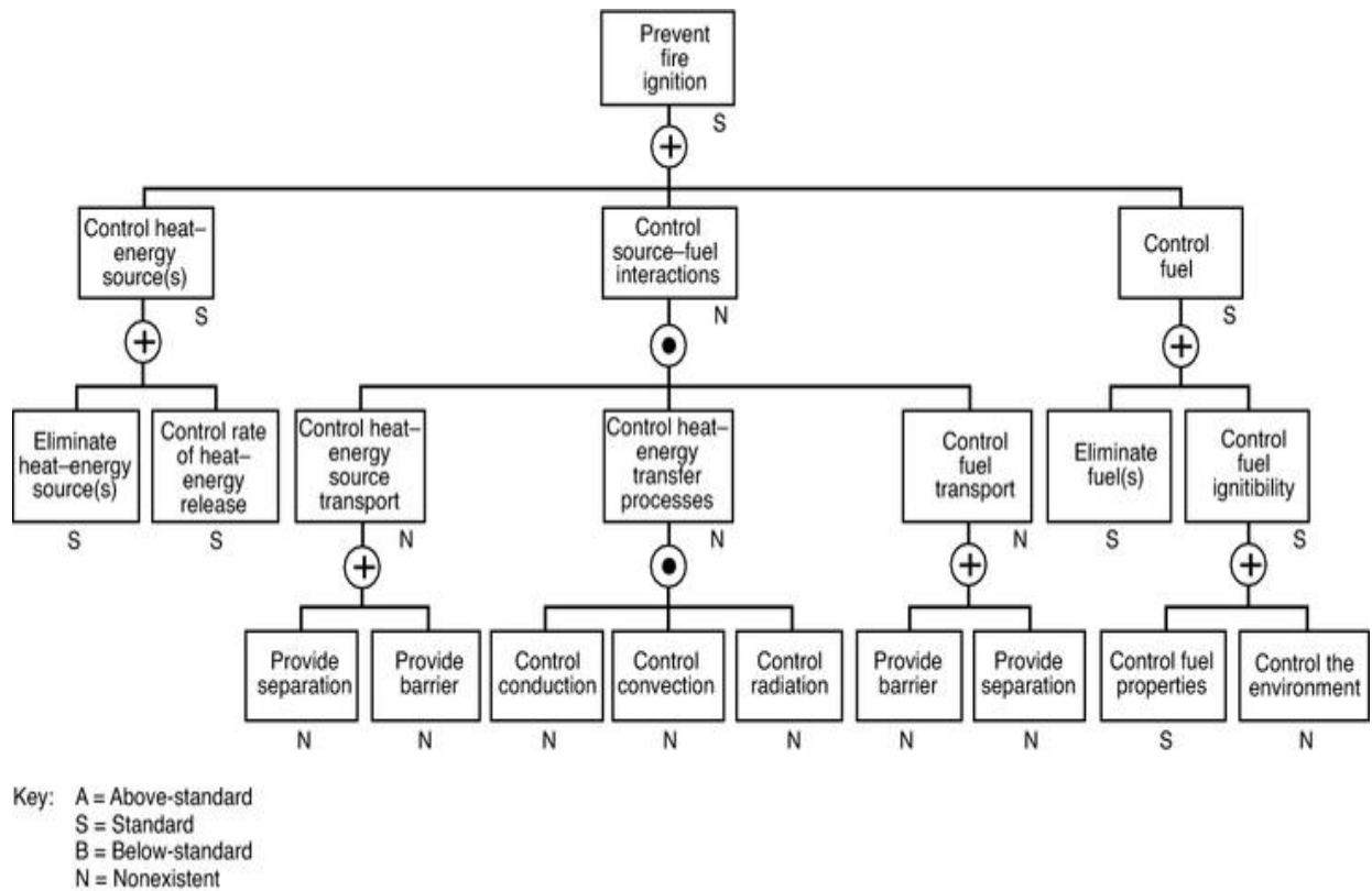
FIGURE 7.3.5 Fire Prevention in a Computer Facility.
