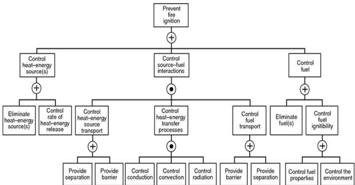
FIGURE 4.4.1 “Prevent Fire Ignition” Branch of Fire Safety Concepts Tree.
