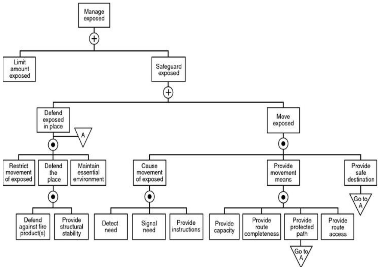
FIGURE 4.5.2.1 “Manage Exposed” Branch of Fire Safety Concepts Tree.
