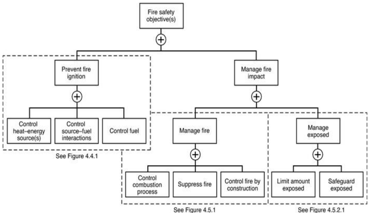
FIGURE 4.3 Top Gates of Fire Safety Concepts Tree with Selected Lower-Tiered Gates.
