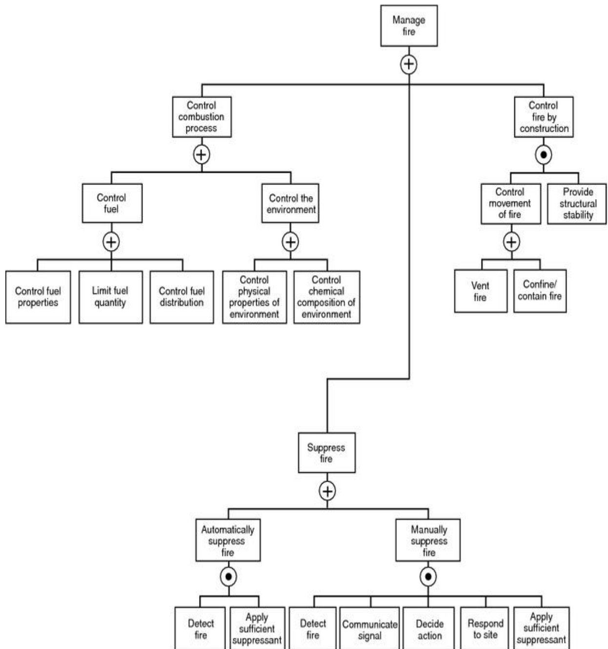
FIGURE 4.5.1 “Manage Fire” Branch of Fire Safety Concepts Tree.
