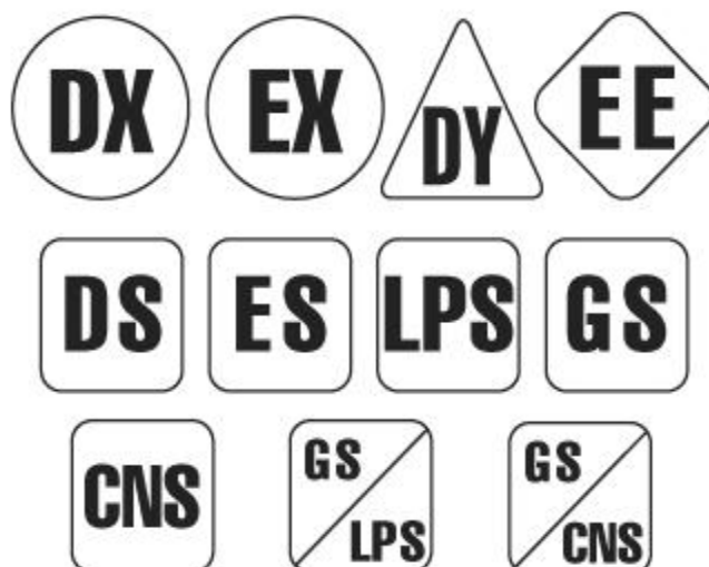
FIGURE 8.4.1.2.1 Markers Used to Identify Types of Industrial Trucks.
