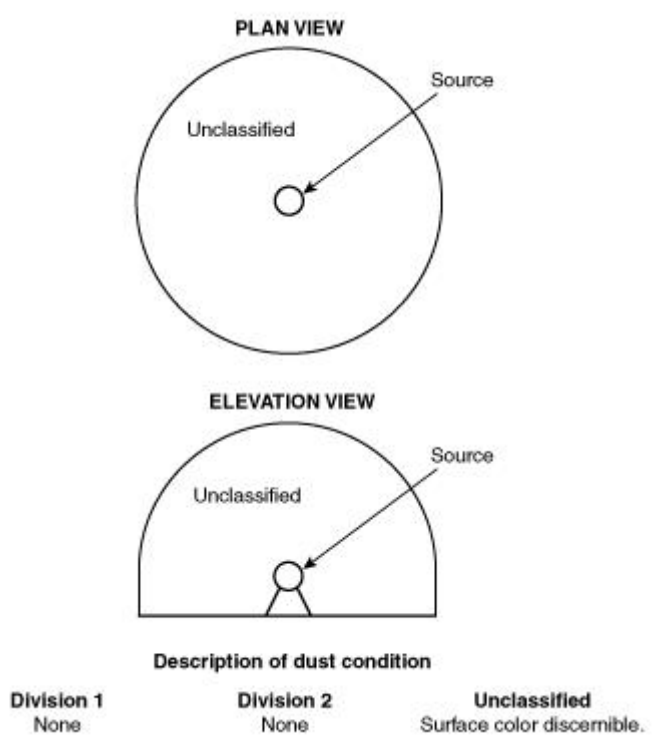
FIGURE 5.8(d) Group F or Group G Dust — Indoor, Unrestricted Area; Operating Equipment Enclosed; Area is an Unclassified Location.
