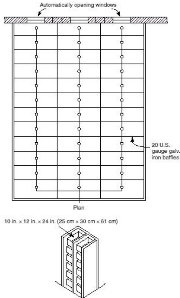
FIGURE 6.7.7 Tote Box Storeroom Showing Arrangement of Sprinklers and Baffles and Section of Tote Box Storage Rack.
