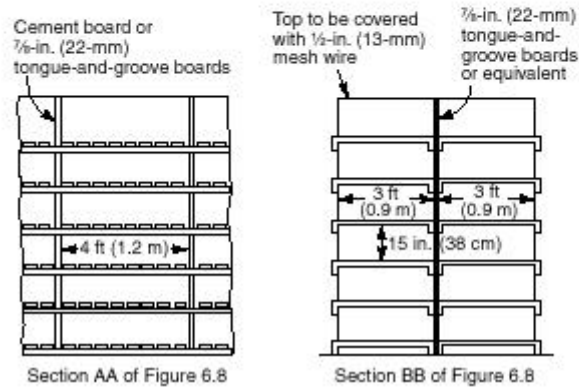
FIGURE 6.8(a) Finished-Stock Storeroom Showing General Arrangement of Racks.
