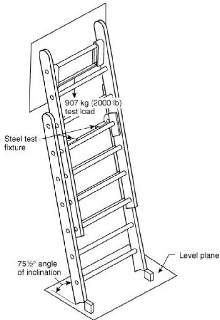
FIGURE 5.4.3.2 Design Verification Pawl Tip Load Test.
