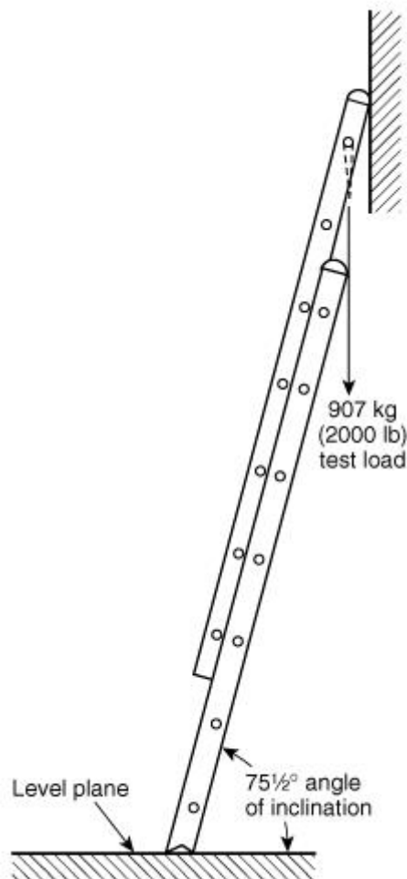
FIGURE 5.4.1.2 Design Verification Beam and Hardware Load Test.
