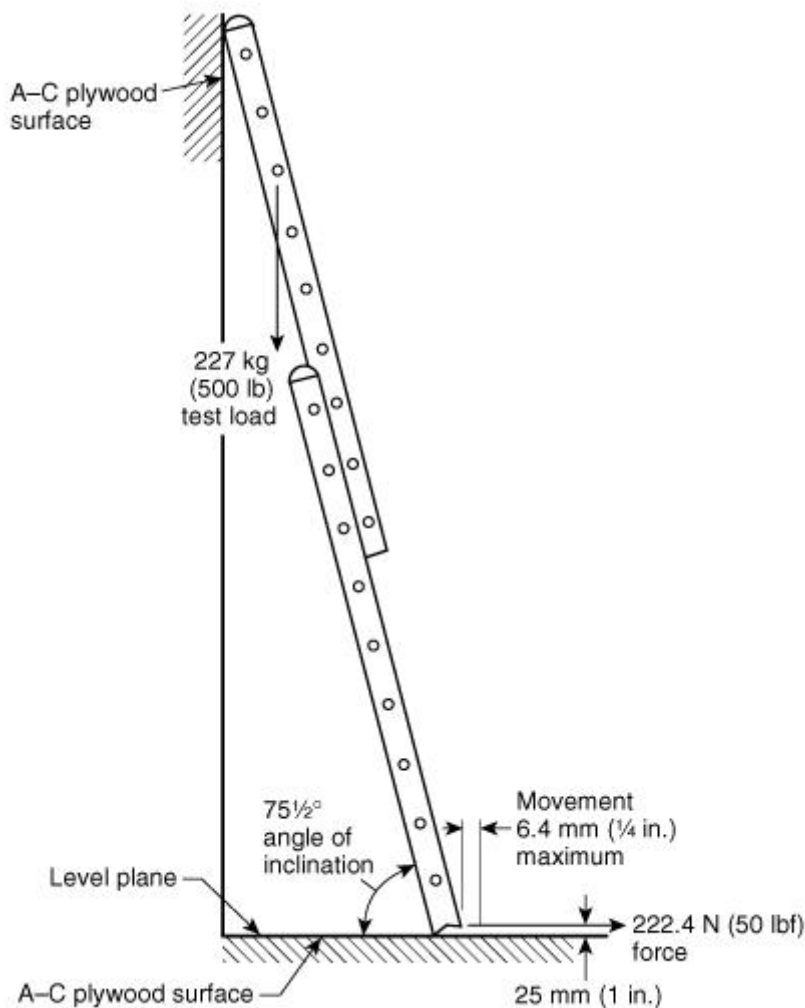
FIGURE 5.2.9.2 Design Verification Butt Spur Slip Test.
