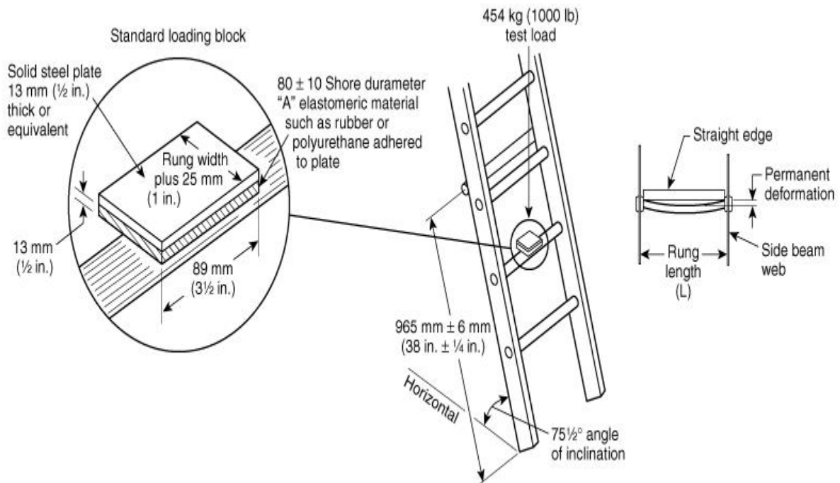
FIGURE 5.2.3.1.1 Design Verification Rung-Bending Test.
