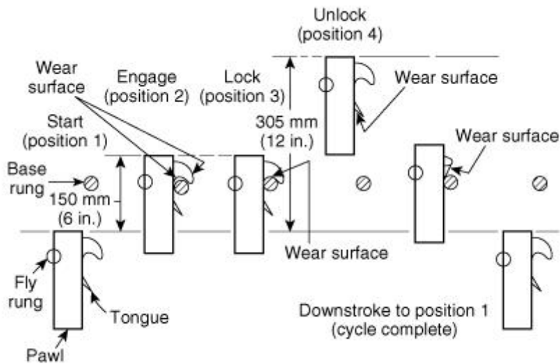
FIGURE 5.5.1.2(b) Design Verification Rung-Pawl Testing Cycle.
