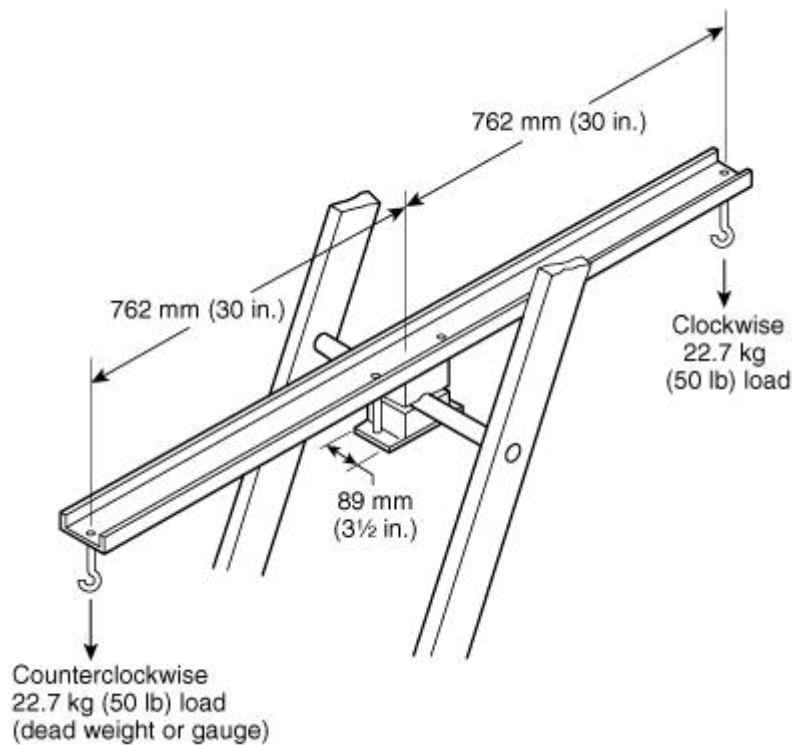
FIGURE 5.2.5.2 Design Verification Rung Torque Test.
