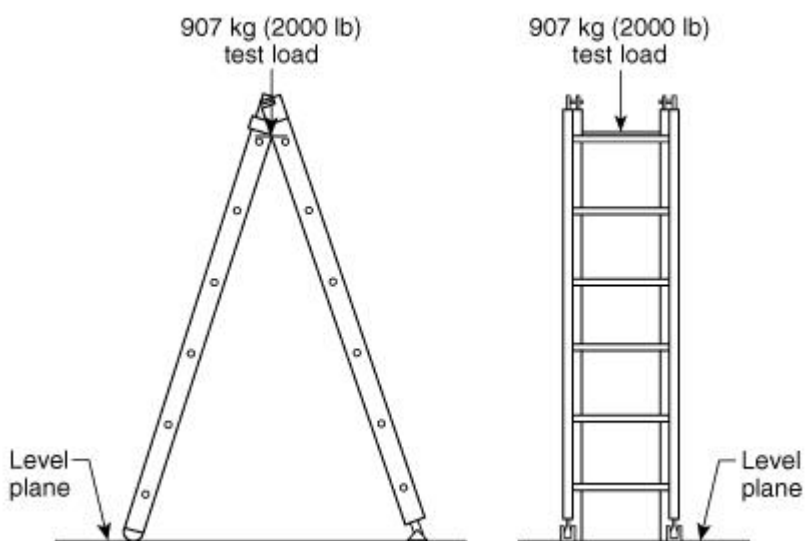
FIGURE 5.6.2.1 Design Verification Combination Ladder Compression Test.
