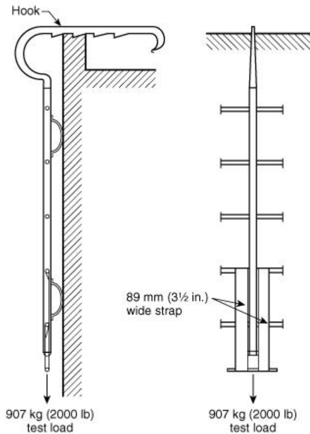
FIGURE 5.8.1 Design Verification Pompier Ladder Test.
