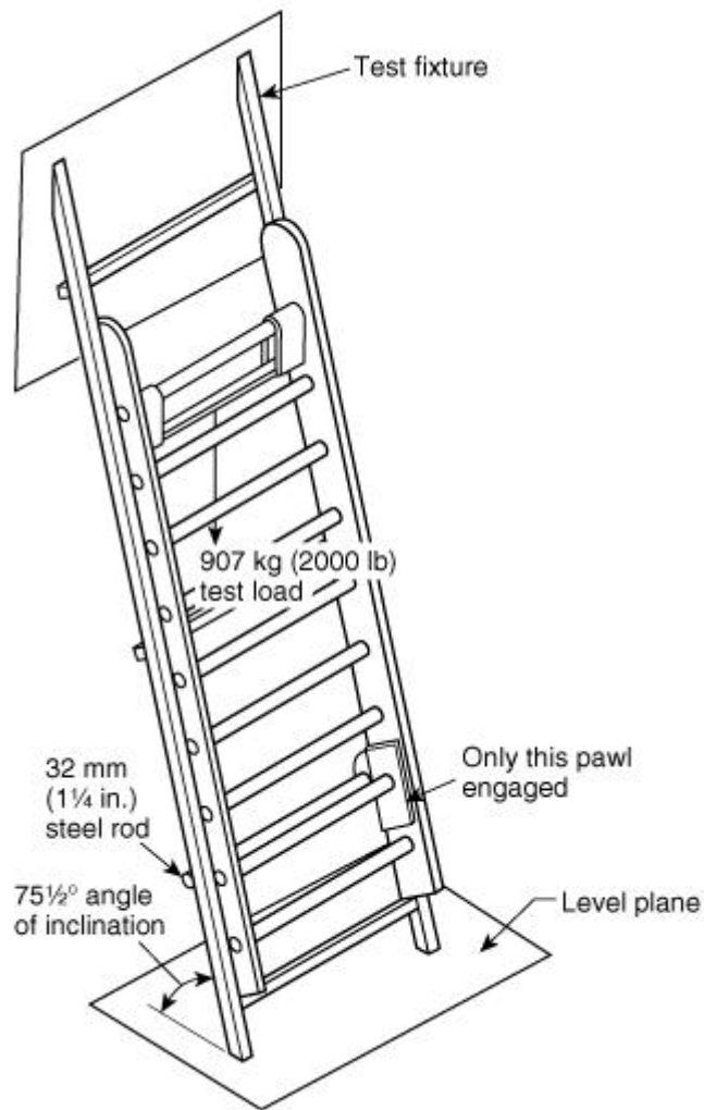
FIGURE 5.4.2.2 Design Verification Single Pawl Load Test.
