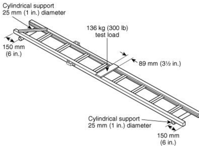
FIGURE 5.7.2.1 Design Verification Folding Ladder Horizontal Bending Test.
