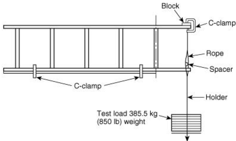
FIGURE 5.2.7.2 Position of Ladder for Design Verification Beam Cantilever-In Bending Test.
