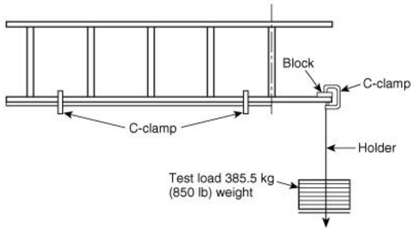
FIGURE 5.2.7.3 Position of Ladder for Design Verification Beam Cantilever-Out Bending Test.
