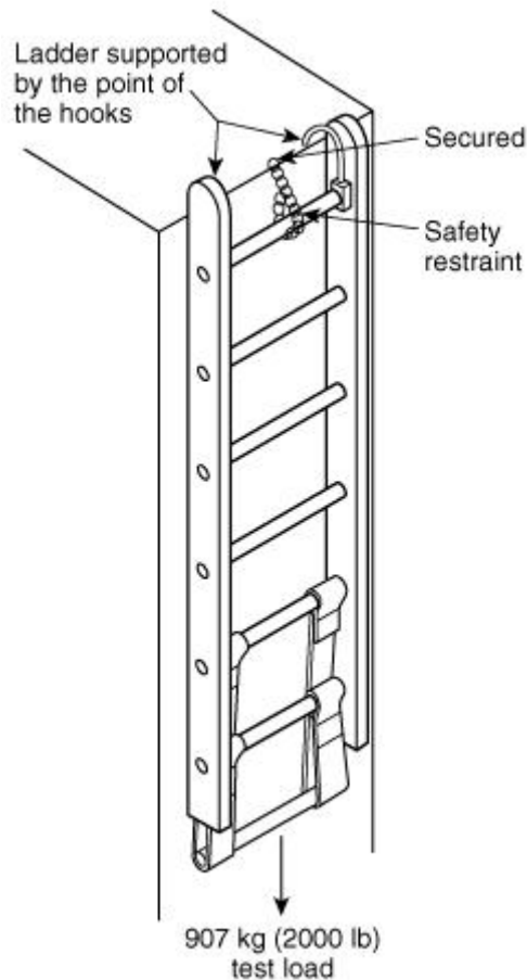
FIGURE 5.3.1 Design Verification Roof Hook Test.
