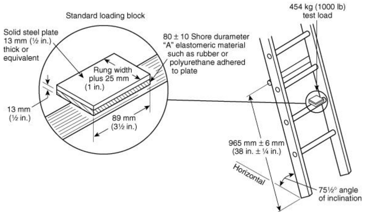
FIGURE 5.2.4.1.1 Design Verification Rung-to-Beam Shear Strength Test.
