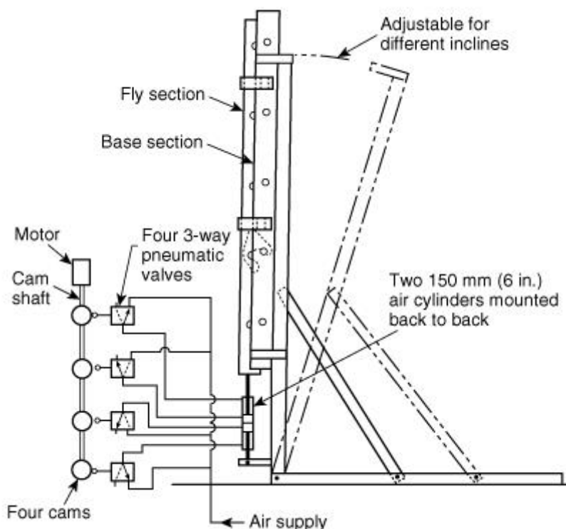
FIGURE 5.5.1.2(a) Design Verification Cyclic Rung–Pawl Test.
